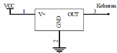
Gbr. 3 Rangkaian Sensor Flow Meter
