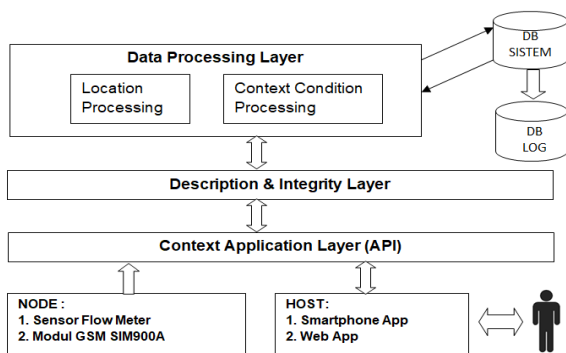
Gbr. 5 Rancangan Service Oriented Architecture
