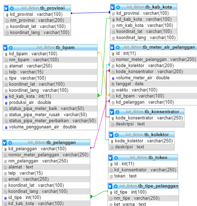
Gbr. 4 Diagram Relasi Tabel
