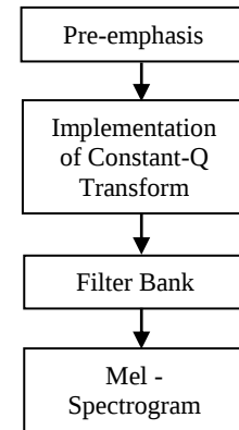
Fig. 4. Improved MFCC.
