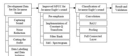
Fig. 1. Research flows.
