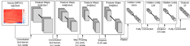
Fig. 5. CNN model.
