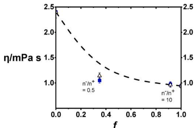
Fig. 11. Viscosity ( \eta ) at 25 °C of the supernatants of centrifuged CS + ALG21 mixtures as a function of the original mass fraction of ALG21 ( f ) in the system. The dashed curve represents the data for the unloaded system, taken from Fig. 7b. The blue filled squares indicate the \eta values for the PECs loaded with BAPs, the open triangles the unloaded (but re-suspended) PECs.
