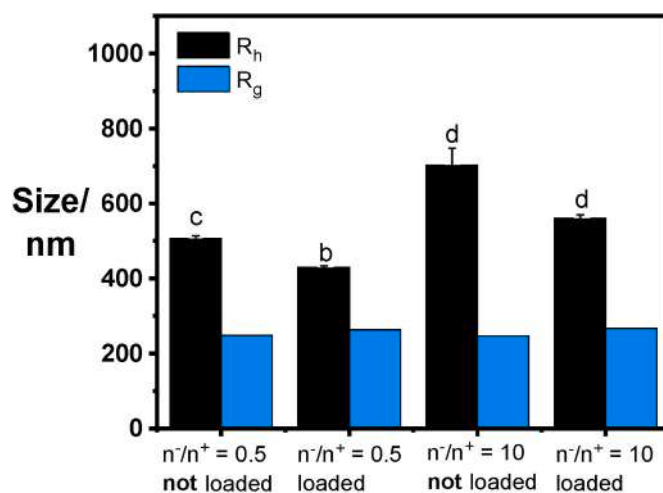
Fig. 6. Measured PEC sizes via DLS ( R_h , black) and SLS ( R_g , blue) for the CS + ALG21 systems at n^-/n^+ = 0.5 and 10, both loaded and unloaded with BAPs. (Bars with different letters are values that are statistically different from one another, at p < 0.05 ).
