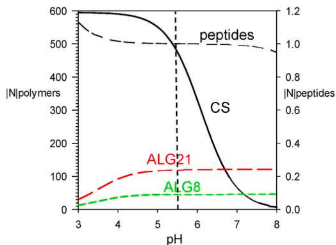
Fig. 4. The magnitude of the net charge |N| on single molecules of the polymers and the BAPs as a function of pH. Left hand ordinate: |N| (+ve) for CS (full black line); |N| (-ve) for ALG21 (red long dashed line); |N| (-ve) for ALG8 (green short dashed line). Right hand ordinate: |N| for the LKPNM or LKP peptides. (Calculation explained in the text). The vertical dashed line indicates the pH (5.5) of PEC formation.
