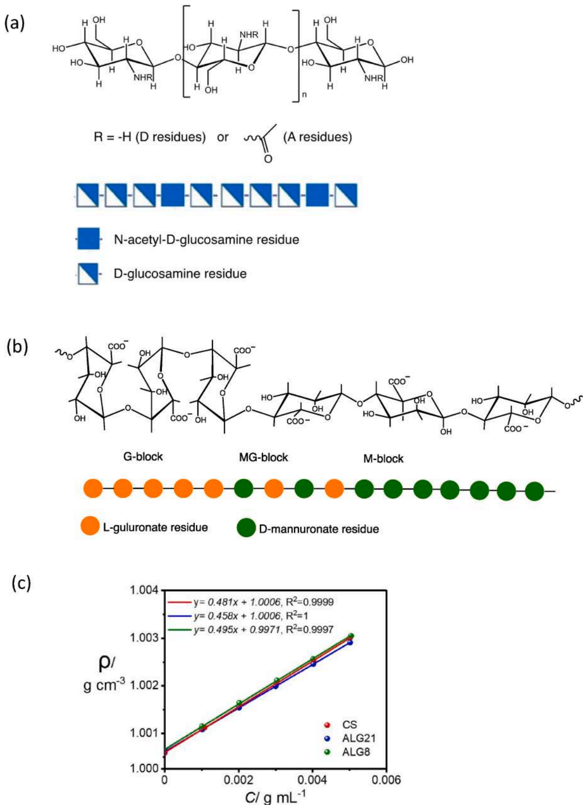
Fig. 1. (a) Chitosan (CS) and (b) alginate (ALG) schematic chemical structures, showing the constituent residues and representative sequences using the standardised symbol nomenclature for glycans (chitosan: filled blue boxes = A residues, half-filled blue boxes = D residues; alginate: orange filled circles = G residues, green filled circles = M residues). (c) Standard curves for unfiltered solution density ( \rho ) versus concentration ( C ): CS (red); ALG21 (blue); ALG8 (green), with the corresponding linear regression lines and coefficients shown.
