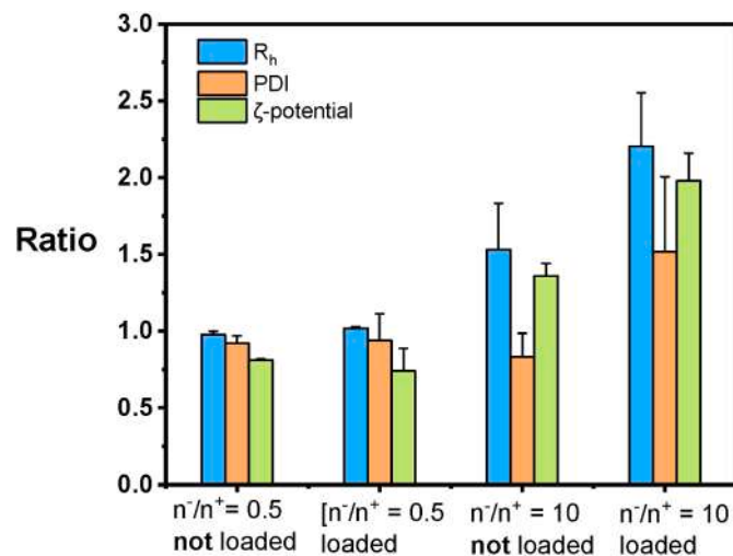
Fig. 10. Ratio between freshly prepared and re-suspended values of R_h , PDI and \zeta of both loaded and unloaded CS + ALG21 PECs, at n^-/n^+ = 0.5 and 10.
