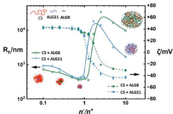
Fig. 5. Hydrodynamic radius ( R_h ) and \zeta -potential of unloaded PECs as a function of molar charge ratio n^-/n^+ at a total polymer concentration of 2 mg mL -1 .
