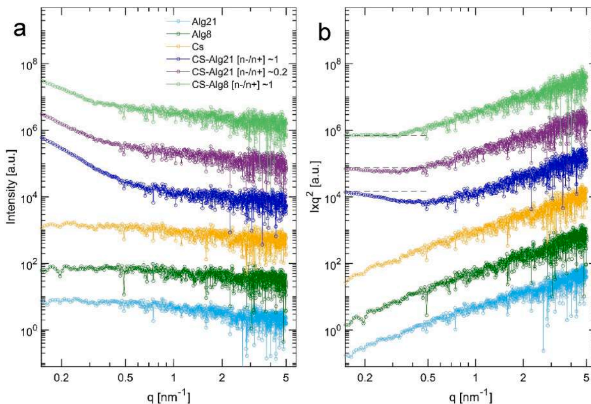
Fig. 8. Small-angle X-ray scattering (SAXS) patterns (a) and corresponding Kratky plots (b) are presented for 2 mg mL -1 CS, ALG, and their PECs at two different n^-/n^+ molar charge ratios. The Kratky plots demonstrate swollen chain behaviour for pure polyelectrolytes, whereas Gaussian and collapsed chains/clustered structures are observed for PECs of ALG8 and ALG21, respectively. The scattering profiles were acquired at 85 mM NaCl and 25 °C. The horizontal dashed lines in the Kratky plots provide a guide for the Gaussian (random coil) chain behaviour at low q values.
