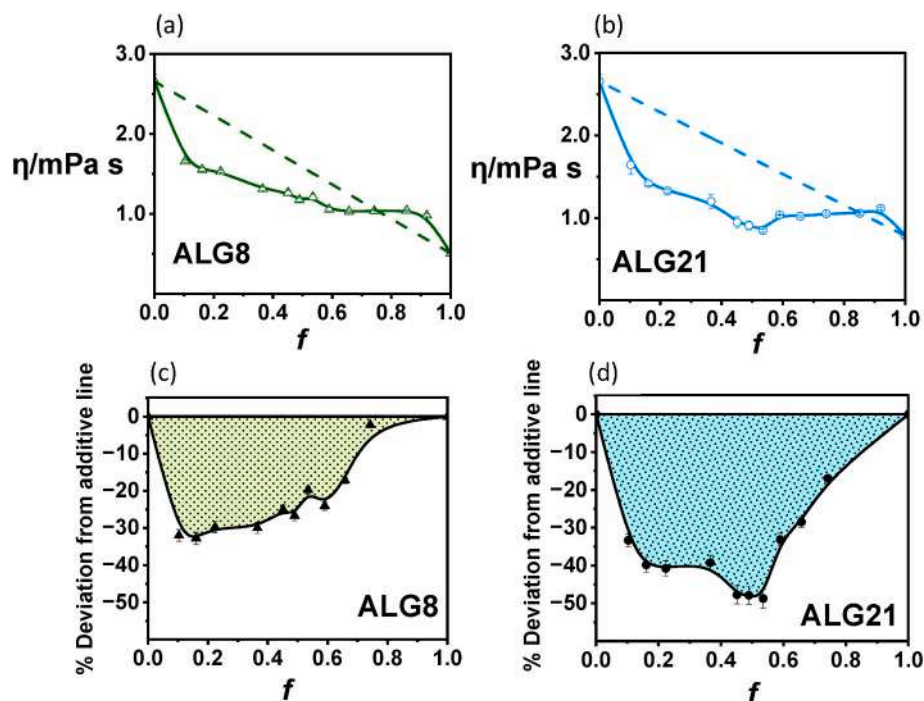
Fig. 7. Viscosity ( \eta ) of the supernatants of centrifuged CS + ALG mixtures as a function of the original mass fraction of ALG ( f ) in the systems for (a) CS + ALG8 and (b) CS + ALG21 at 25 °C. The dashed lines in (a) and (b) are the theoretical \eta of the biopolymer mixtures assuming simple additivity of the \eta of the pure components. (Thus \eta at f = 0 and 1 are the values of CS and ALG stock solutions at 2 mg mL -1 , respectively). Figures (c) and (d) show the % difference of the measured \eta from the additive line for CS + ALG8 and CS + ALG21, respectively.
