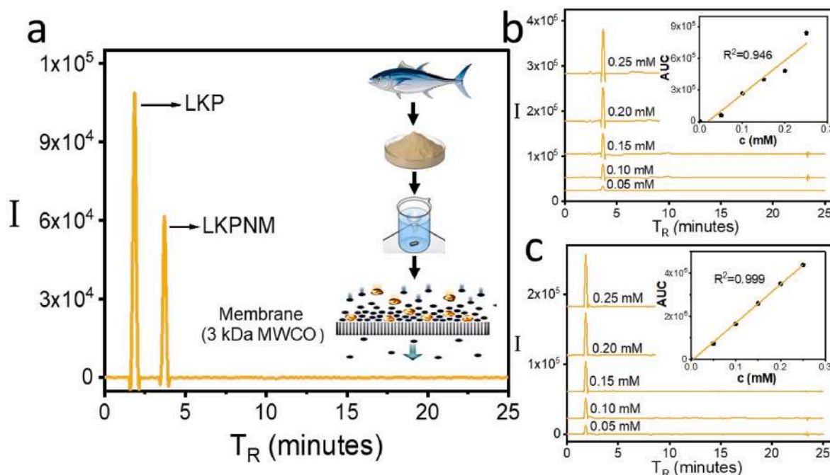
Fig. 3. (a) HPLC chromatograms of \leq 3 kDa PeptACE BAPs and their fractionation scheme. Standard curves for LKPNM (b) and LKP (c) calculated from area under the curves (AUC).
