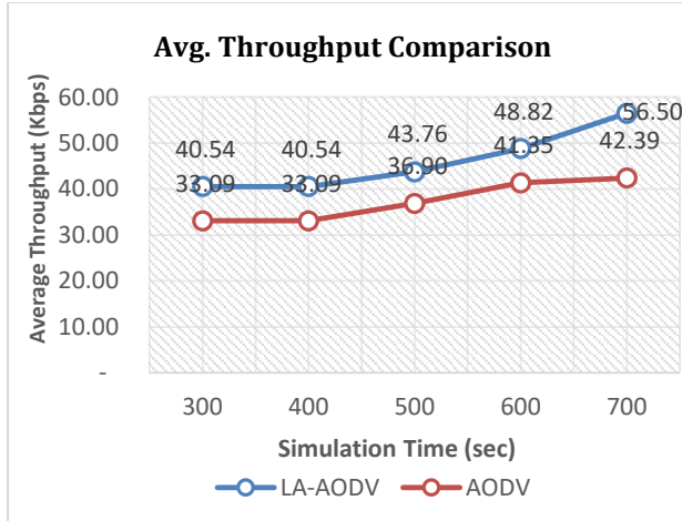
Figure 6. Average Throughput Comparison results for all traffic scenarios within the simulation
