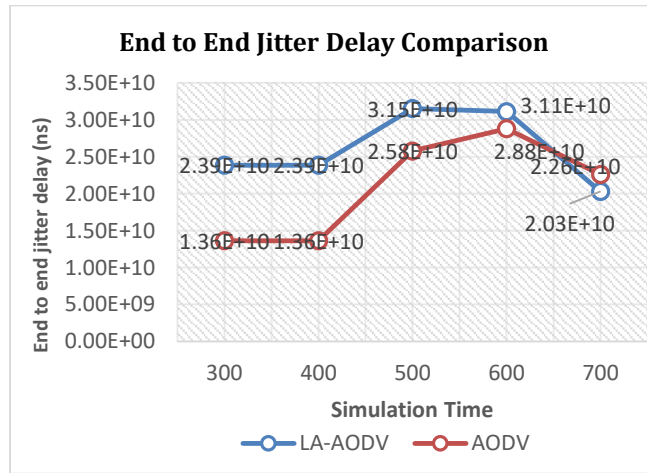
Figure 8. The End-to-End Jitter comparison results for all traffic scenarios within the simulation time range of 300 to 700 seconds
