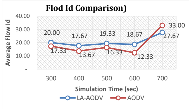
Figure 3. AODV and LA-AODV Flooding ID Comparison across the 300 to 700-second timeframe in V2V communication scenarios
