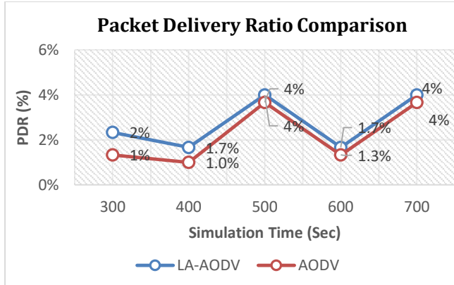
Figure 5. PDR Comparison across the 300 to 700-second timeframe in V2V communication scenarios
