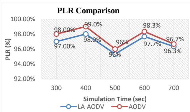
Figure 4. PLR Comparison across the 300 to 700-second timeframe in V2V communication scenarios
