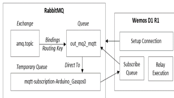
Figure. 3. Diagram of Message Subscribe.
