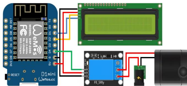
Figure. 4. Hardware Circuit of Edge.
