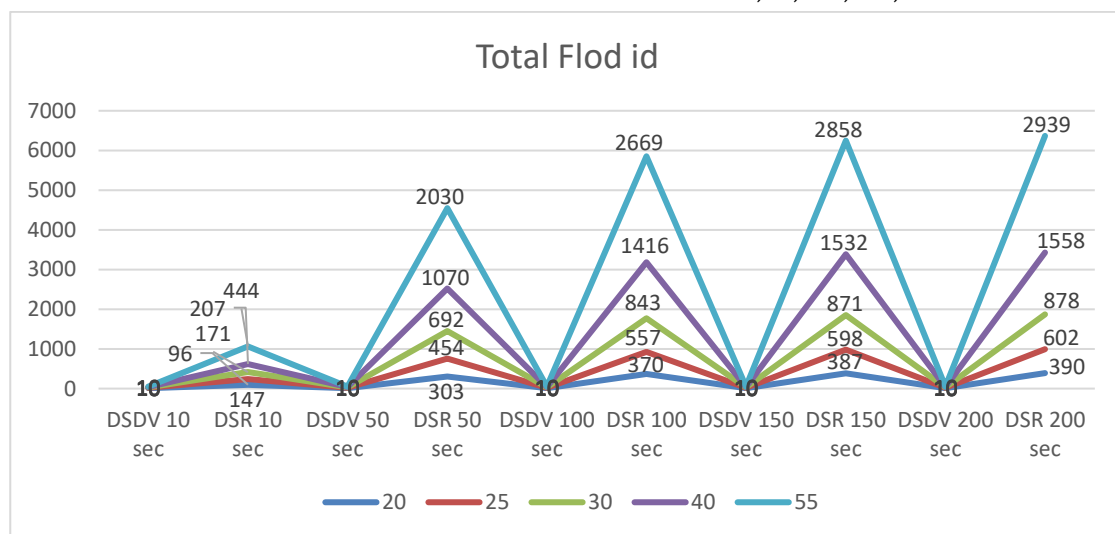
Gambar 3. Perbandingan Total Flood Id
