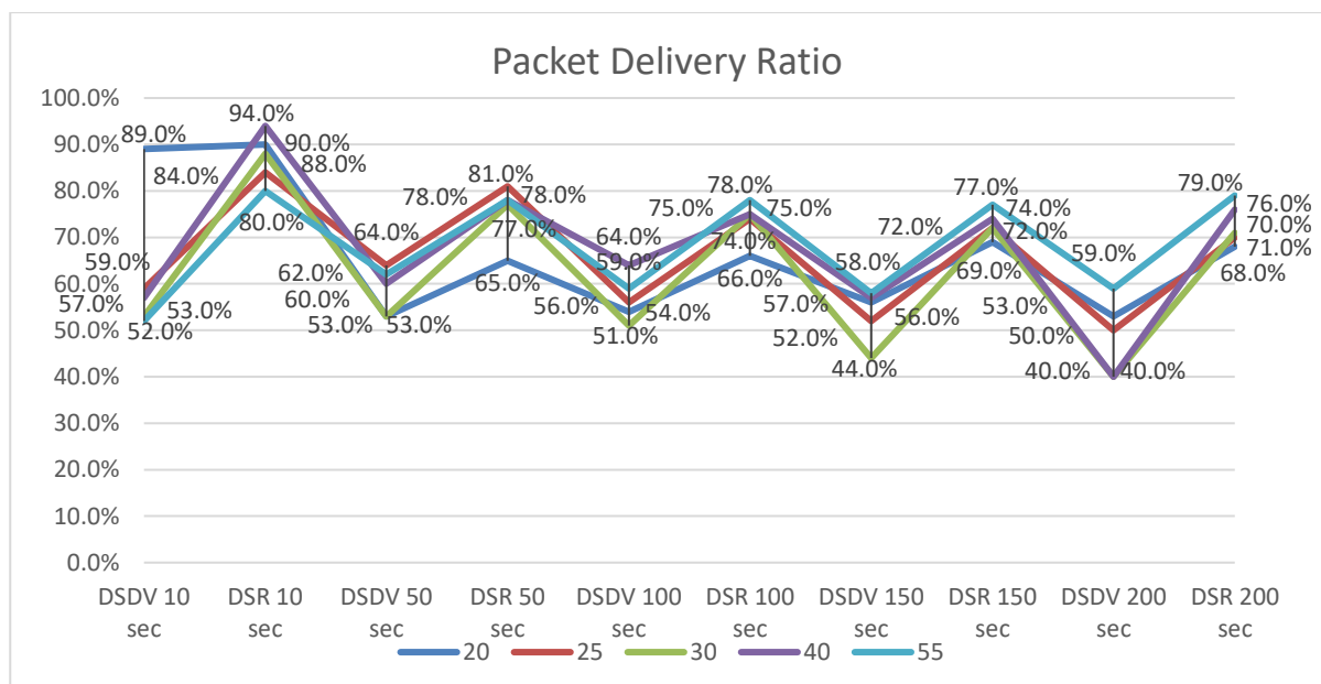
Gambar 5. Perbandingan Packet Delivery Ratio
