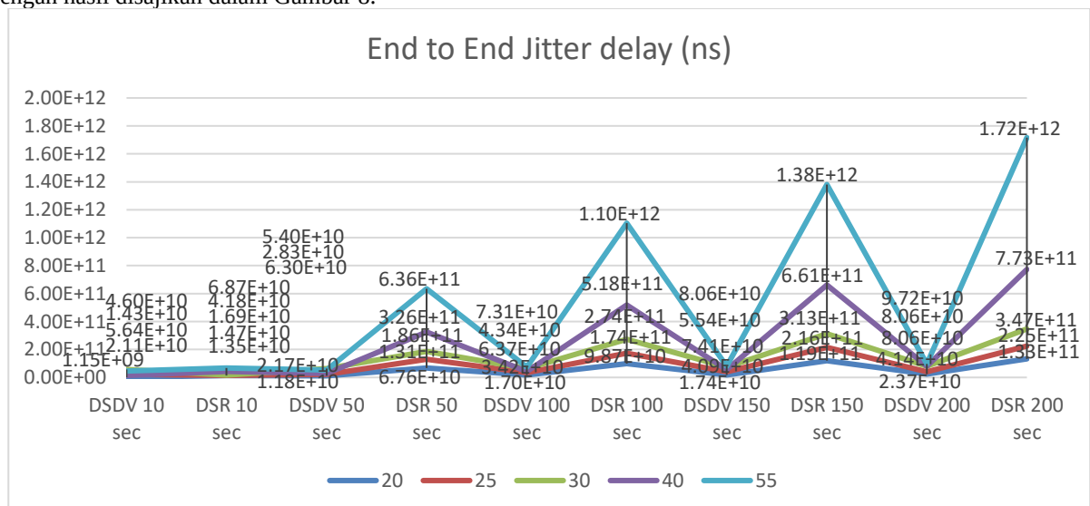
Gambar 8. Perbandingan End to End Jitter Delay (ns)
