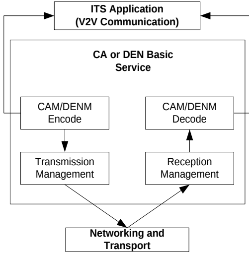
Figure 2. CA and DEN basic service to support ITS-S in ETSI facilities layer
