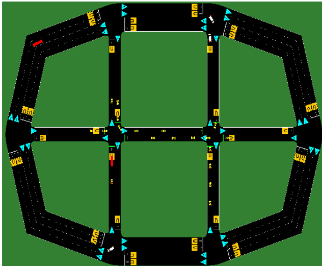
Figure 3. A Modification Offline Network Map in SUMO
