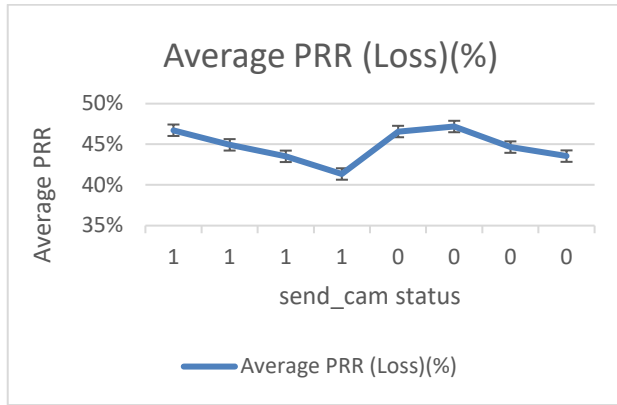
Figure 5. Average PRR Result
