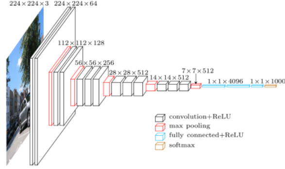
Fig. 7. VGGNet CNN Model Architecture
