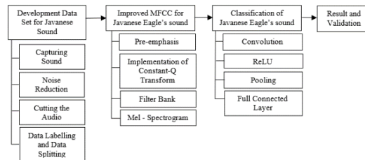
Fig. 1. Research Flows
