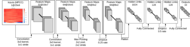
Fig. 5. CNN Model
