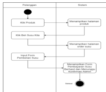
Gambar 5. Activity Diagram Beli Produk
