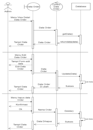
Gambar 9. Sequence Diagram Mengelola Data Order
