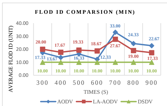
Figure 6. This study analyzes AODV, LA-AODV, and DSDV's Flood ID behavior in V2V communication (300-900 seconds).
