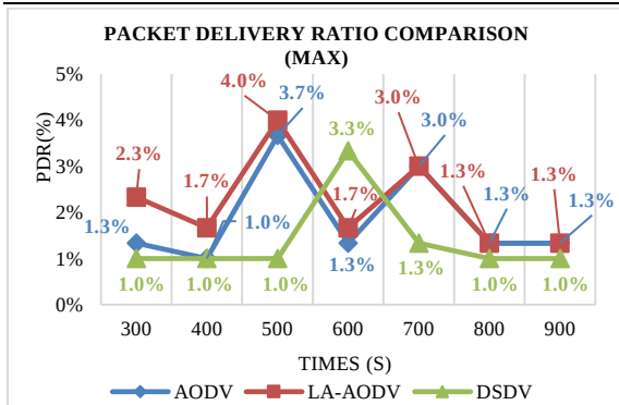
Figure 8. This research explores Packet Delivery Ratio (PDR) in V2V communication for AODV, LA-AODV, and DSDV between 300 and 900 seconds.
