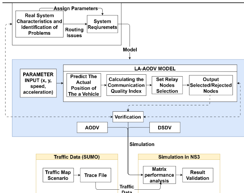
Figure 3. This study analyzes routing protocols in V2V simulation design.
