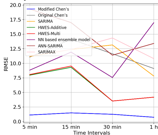
Fig. 2 Score of RMSE
