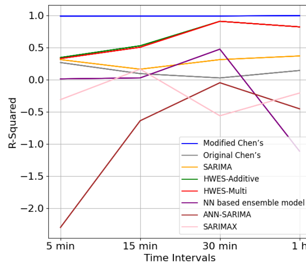
Fig. 3 Score of R-Squared
