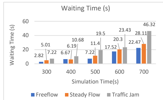
Figure 8. Displays higher waiting times with increased node counts, particularly in traffic jam.
